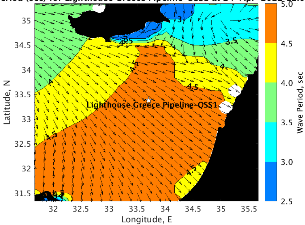
Period (sec) for Lighthouse Greece Pipeline-OSS1 at 24-Apr-2022 12:00:01
